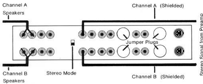
CS-1200 PATCH DIAGRAM 1 Stereo Operation Unbalanced High Z Inputs (Typical Home Stereo)
